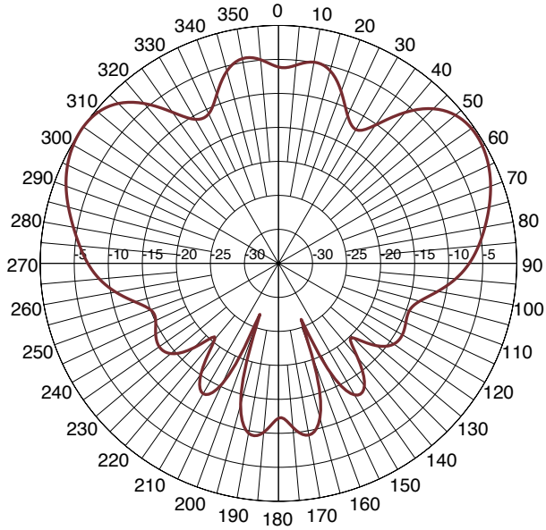
Elevation Pattern at 850MHz
