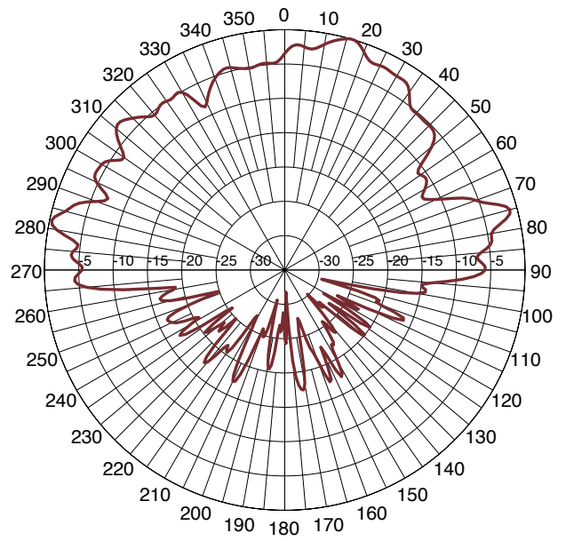
Elevation Pattern at 5400MHz
