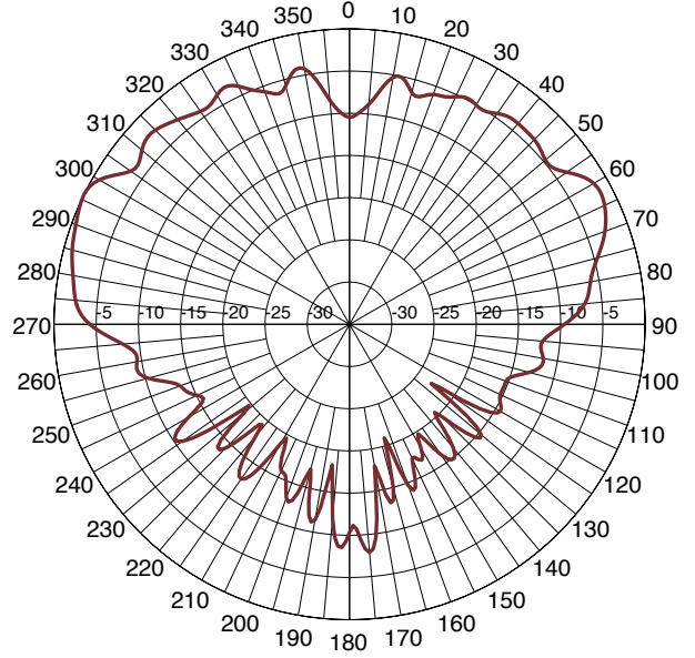
Elevation Pattern at 1900MHz
