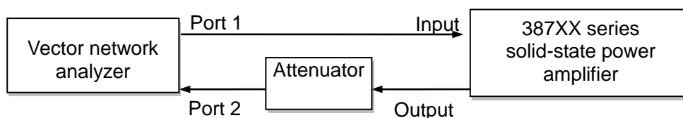
Figure 5-1 Gain and standing wave testing diagram
