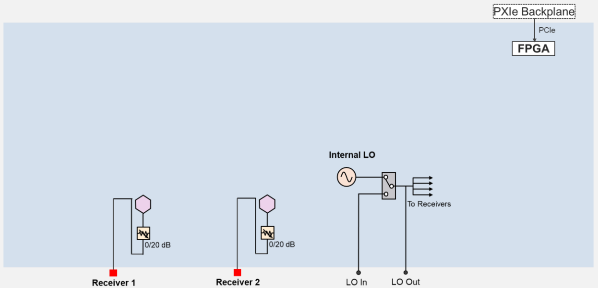
M981xA PXIe Receiver Module (Included in Option 491 or 691)
