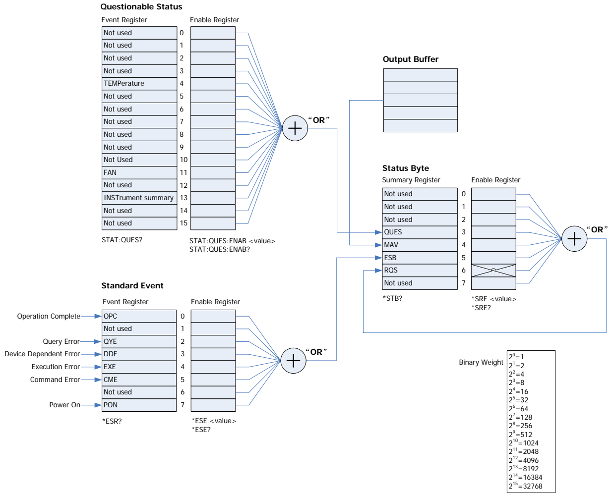
Figure 1-2 The SCPI Status System of DP800 Series Multi-channel Models (Take DP831A as an Example)
