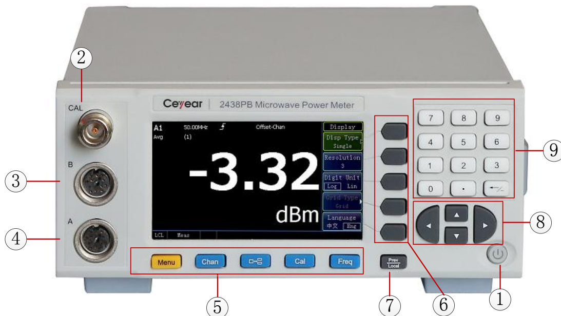
Fig. 3.9 Front Panel of Instrument
