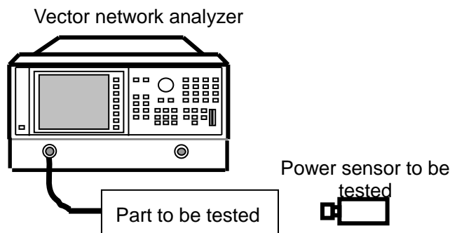
Fig. 8.8 Sensor SWR Test Block Diagram
