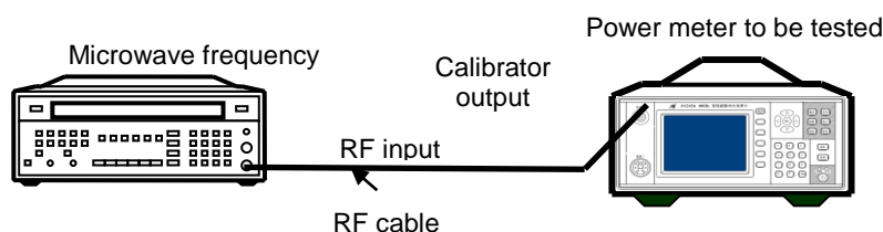
Fig. 8.3 Calibrator Frequency Accuracy Test Block Diagram
