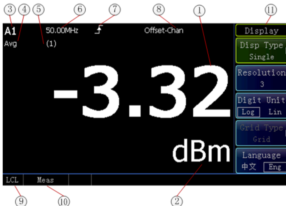
Fig. 3.11 Measurement Interface in case of Connection with a Peak Power Sensor
