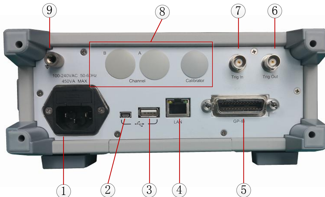
Fig. 3.10 Rear Panel of Instrument
