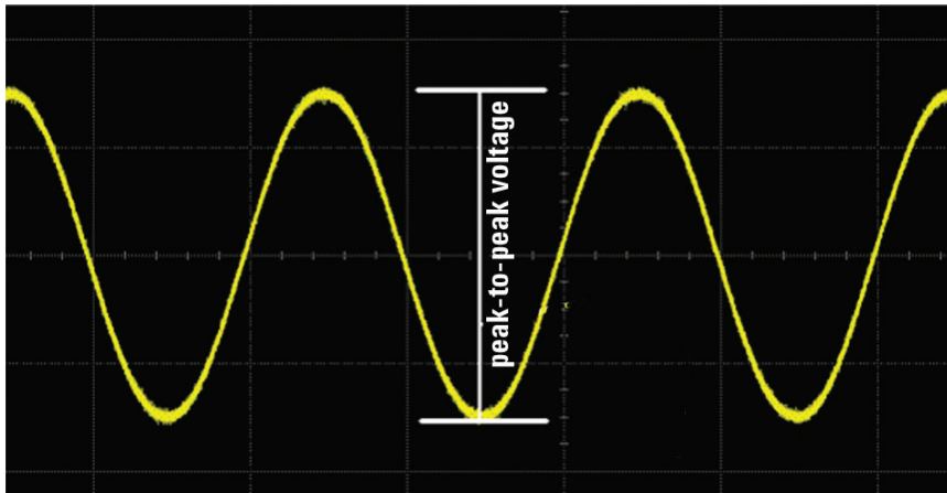
Figure 23. Peak-to-peak voltage.
