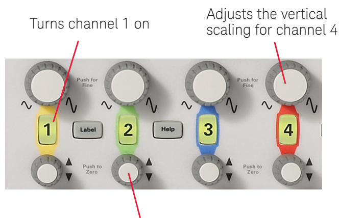
Figure 16. Front panel vertical control section on a Keysight InfiniiVision 2000 X-Series oscilloscope.
