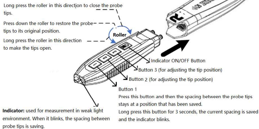
Figure 11 How to Operate the Hand-held Differential Probe Head
