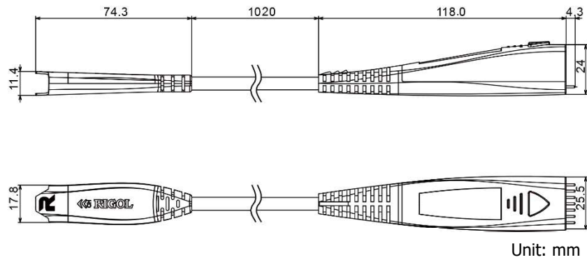
Figure 1 Probe Dimensions
