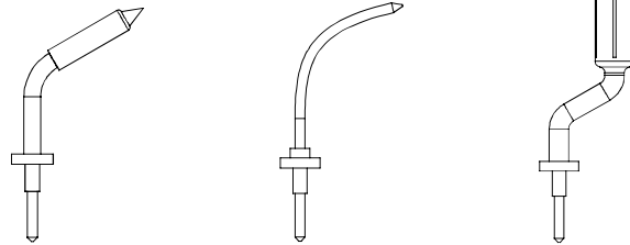
(d) Ground Pin (pogo) (e) Ground Pin (solderable) (f) Ground Adapter (square pin)
