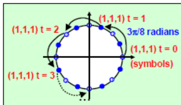
Fig. 10 Diagram of EDGE vectors
