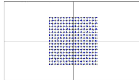
Figure 2.21 1024QAM
