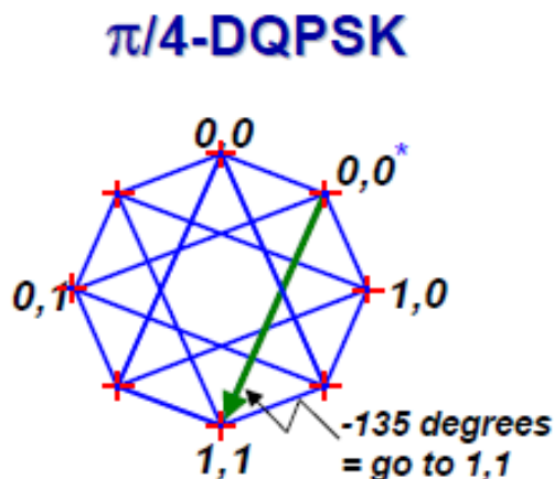
Fig. 7 Combined constellation
