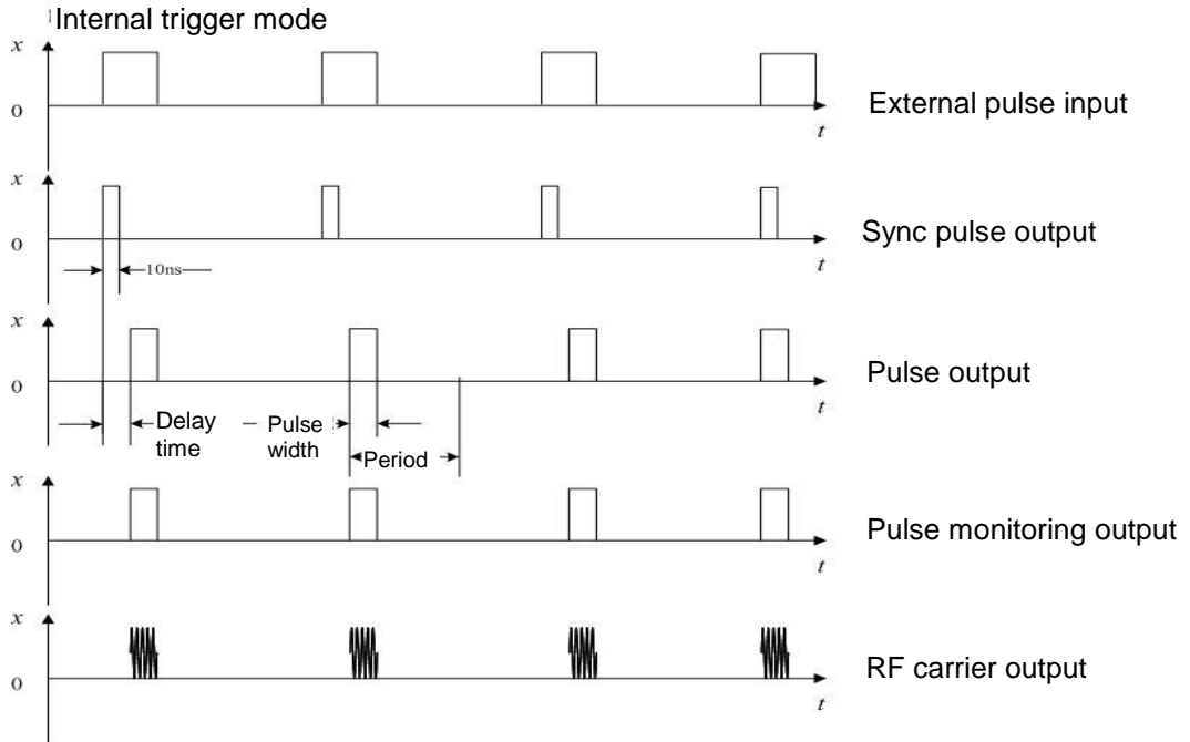
Figure 4.19 Internal trigger mode
