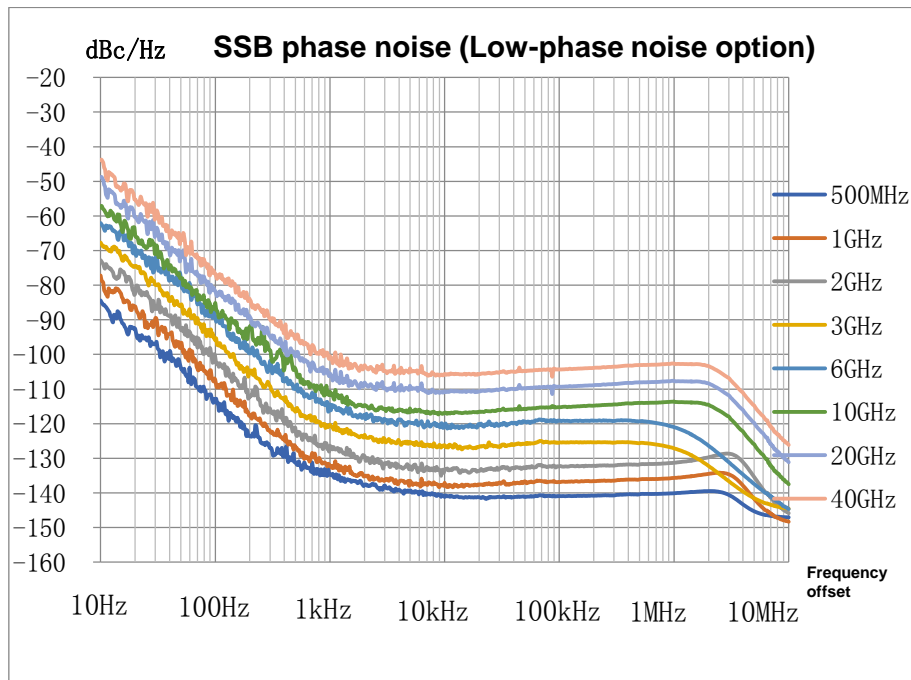
Figure 2.4 SSB phase noise (non-V)
