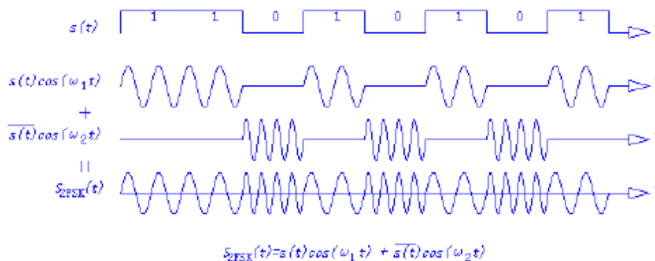
Fig. 1 Schematic diagram of 2FSK
