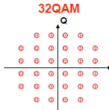
Fig. 6 32QAM constellation
