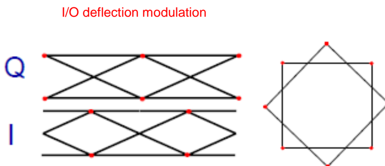
Figure 8 QPSK modulation type
