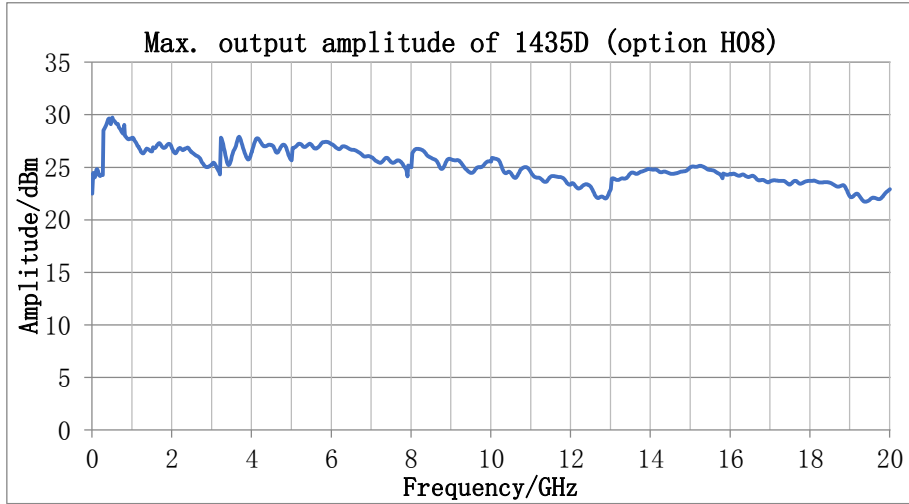
Figure 2.1 Max. output amplitude of 1435D
