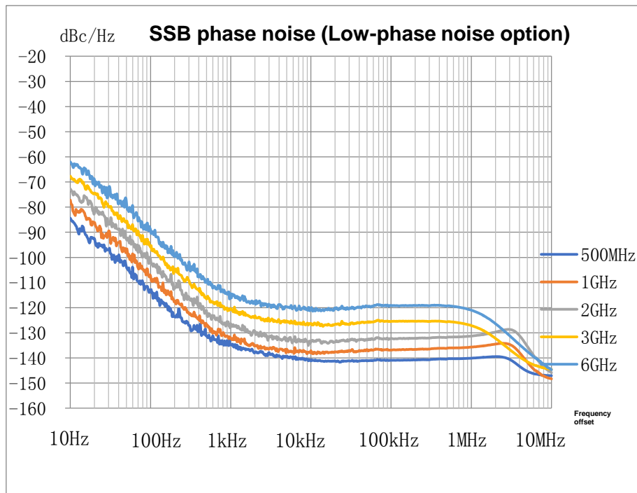
Figure 2.5 SSB phase noise (-V)
