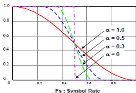
Fig. 11 Diagram of relationship between channel bandwidth and \alpha
