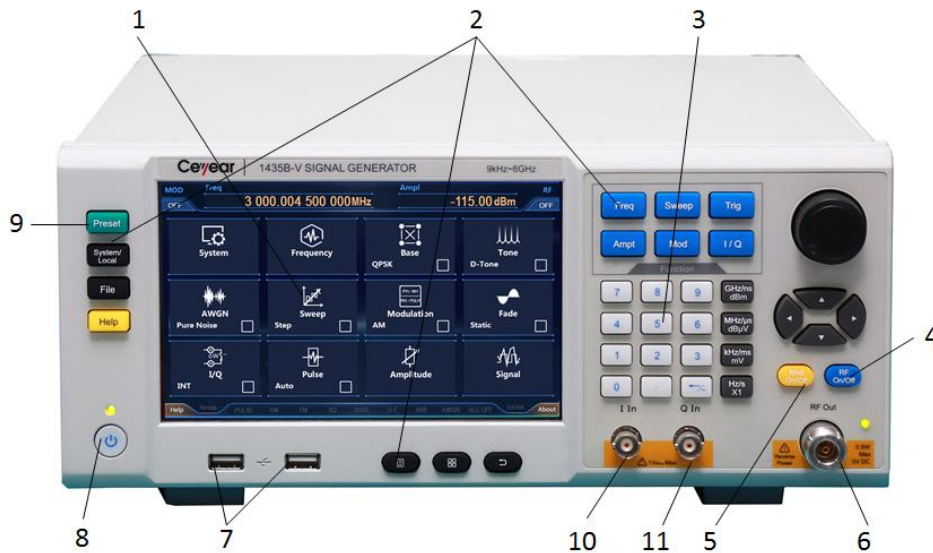
Figure 3.11 Front Panel
