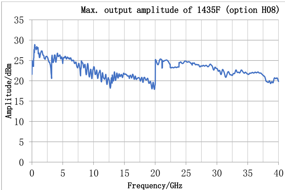
Figure 2.2 Max. output amplitude of 1435F
