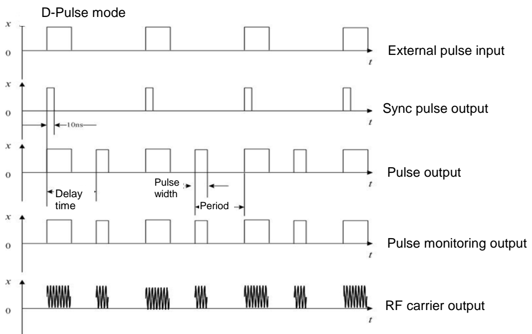
Figure 4.21 D-Pulse mode
