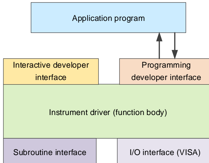
Fig. 6.7 Instrument driver structure model
