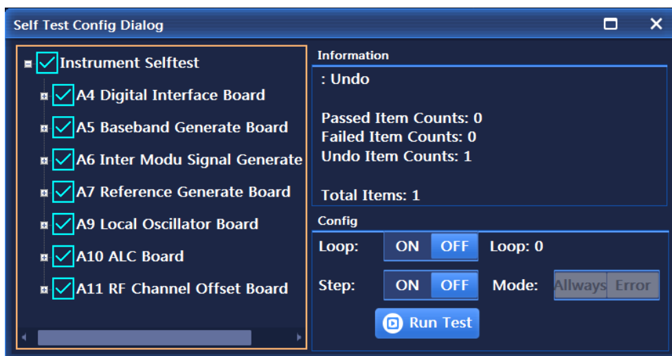
Figure 5.49 Self-test interface
