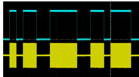
Figure 2.8 Pulse width of 20ns
