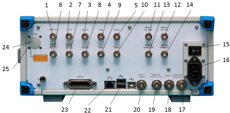
Figure 3.12 Real panel
