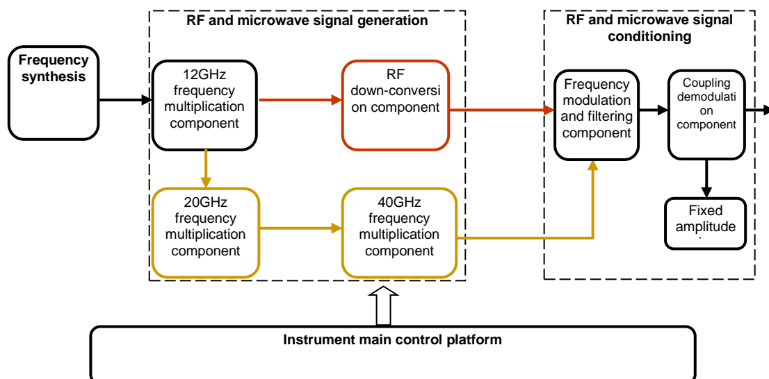
Fig. 7.1 Instrument hardware planning block diagram
