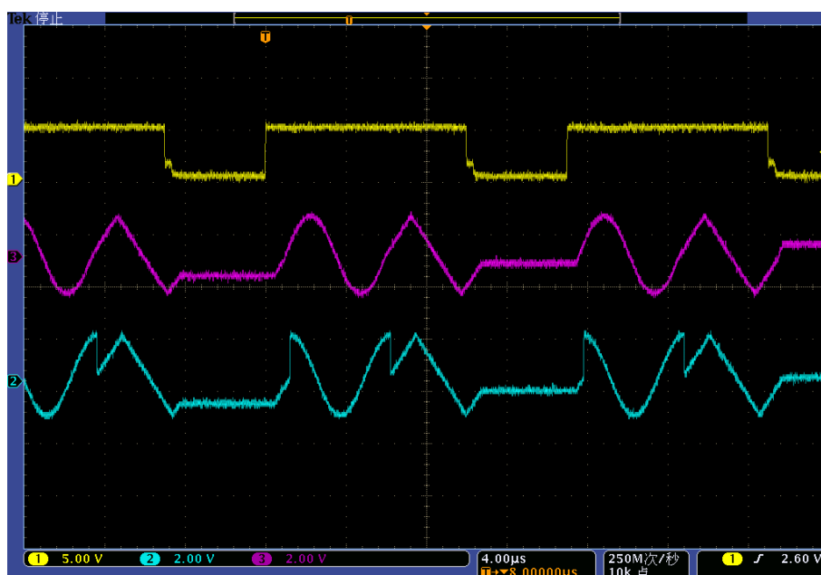
Figure 4.31 Arbitrary wave triggering (Gate Height)
