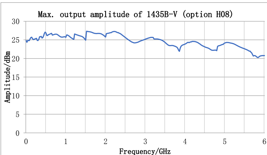
Figure 2.3 Max. output amplitude of 1435B-V
