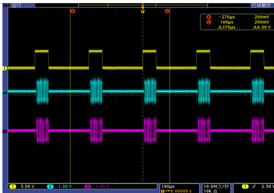
Fig. 4.22 Diagram of Baseband Triggering (Gate/High)
