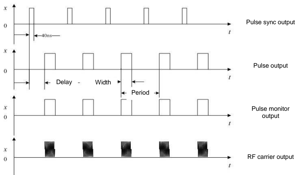
Fig. 4.16 Internal Auto Mode
