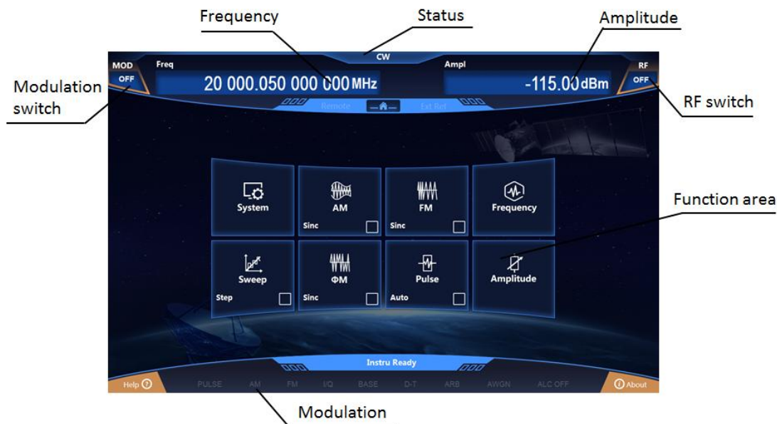
Fig. 3.13 Operating Interface
