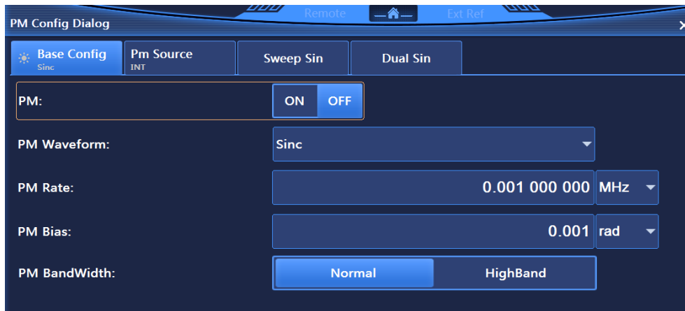
Figure 5.23 Base Config Dialog
