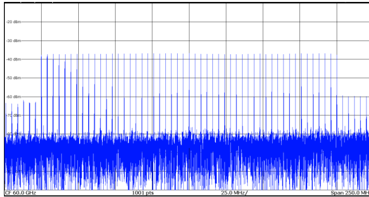
Fig. 2.6 60GHz Carrier 200MHz Modulation Bandwidth Multi-tone Signal
