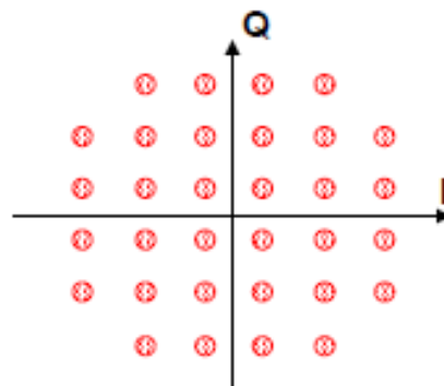
Attached Figure 6 32QAM Constellation
