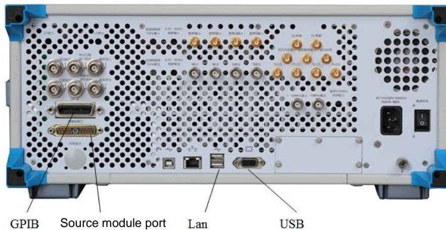
Fig. 2.13 Remote interfaces
