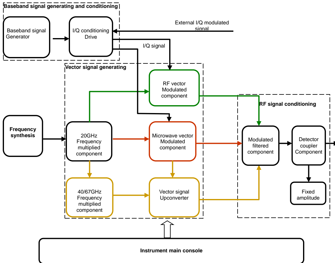
Fig.7.1 Block diagram of instrument hardware overall plan
