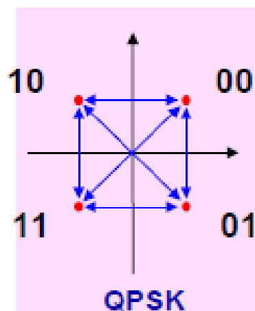
Attached Figure 3 QPSK Diagram
