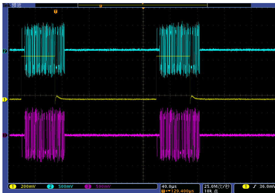
Fig. 4.21 Diagram of Baseband Triggering (Continues/Single)
