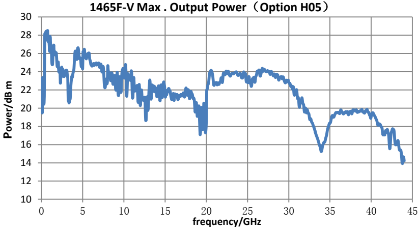
Fig. 2.4 Max. Output Power of 1465F-V+H05
