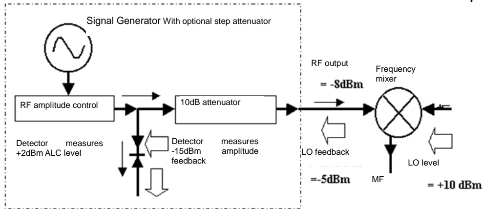
Fig. 4.12 Effects of Reverse Power (-8dBm Non-coupling Output)
