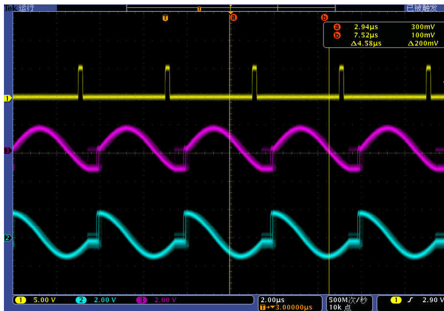
Fig. 4.24 Diagram of Arbitrary Trigger (Continue/Realtime)
