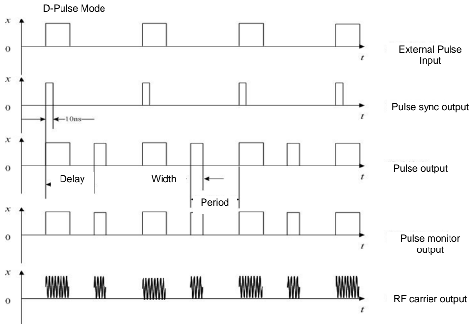
Fig. 4.19 D-Pulse Mode
