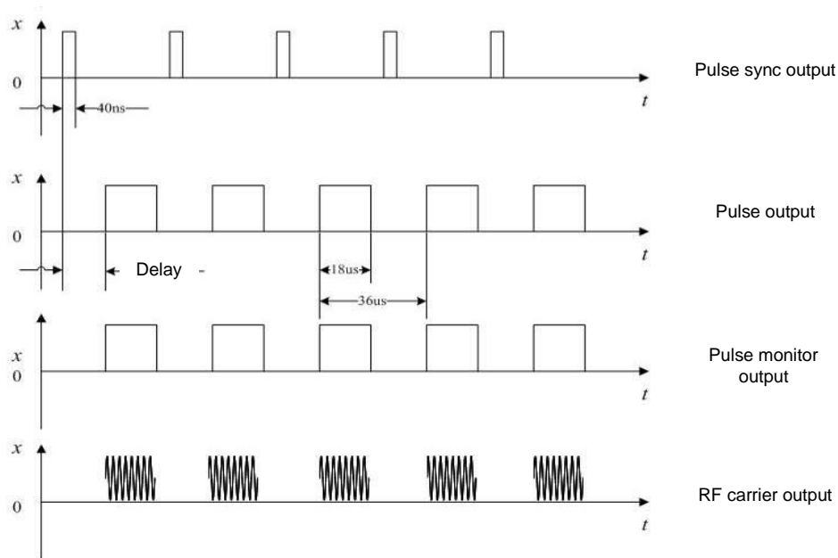
Fig. 4.15 Internal Scalar Pulse
