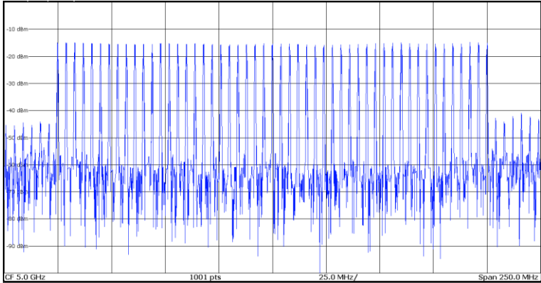
Fig. 2.5 5GHz Carrier 200MHz Modulation Bandwidth Multi-tone Signal
