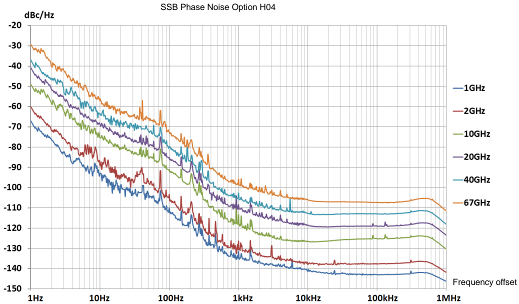
Fig. 2.1 SSB Phase Noise
