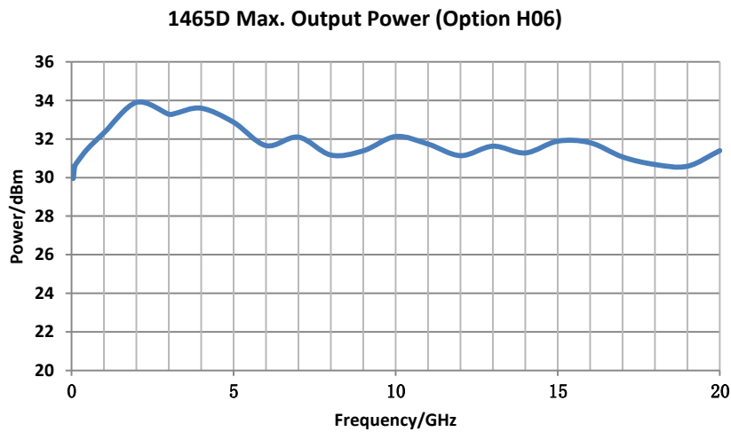
Fig. 2.2 Max. Output Power of 1465D+H06
