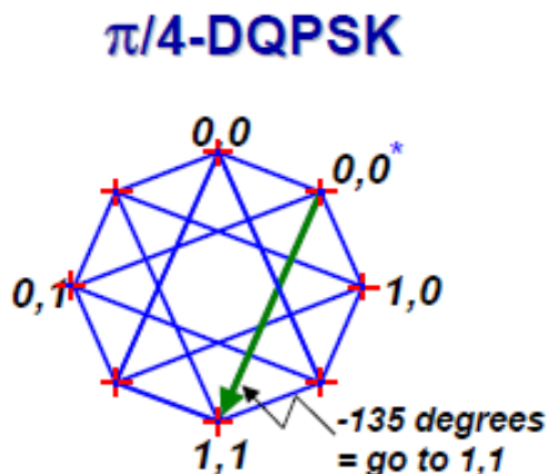
Attached Figure 7 Synthesized Constellation
