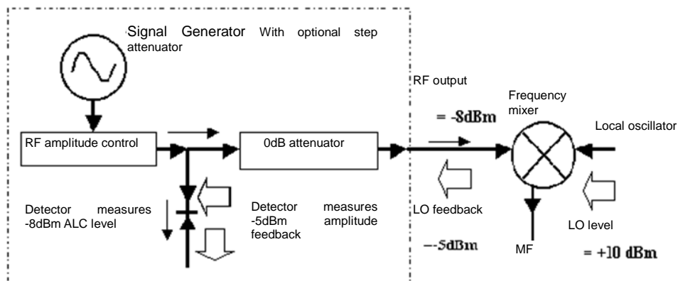
Fig. 4.11 Effects of Reverse Power ( -8\text{dBm} Coupling Output)
