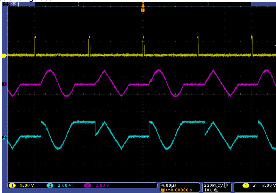
Fig. 4.28 Diagram of Arbitrary Trigger (Wave Seg Single)
