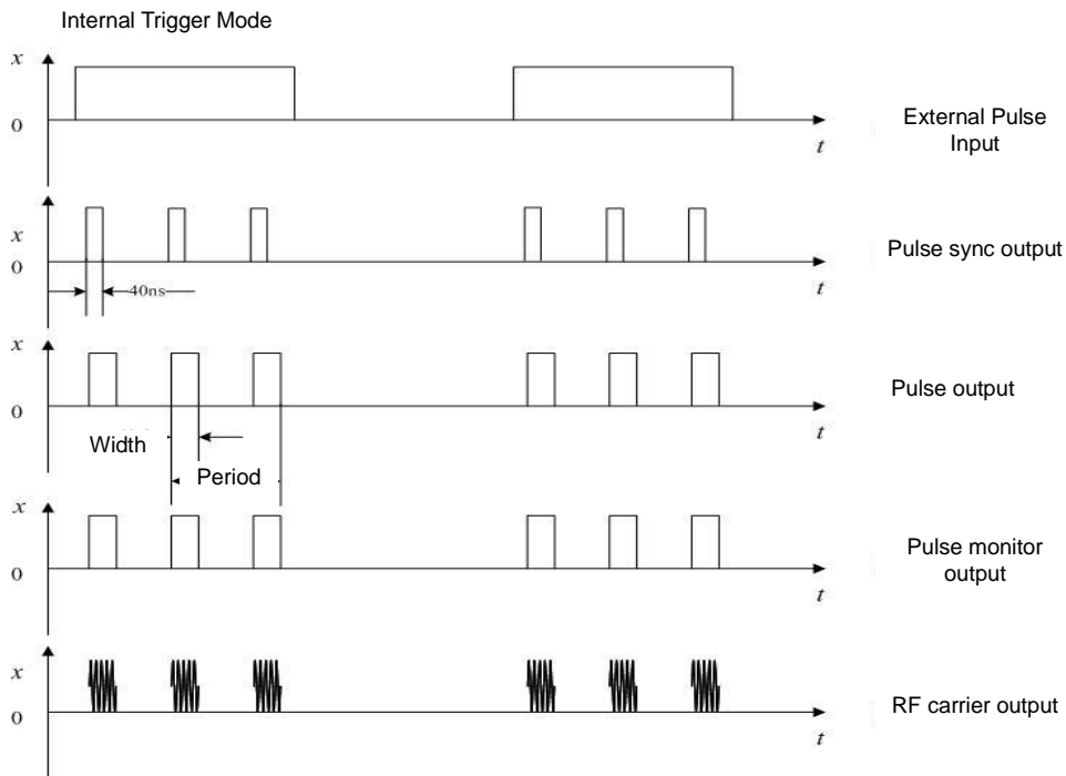
Fig. 4.18 Internal Gate Mode
