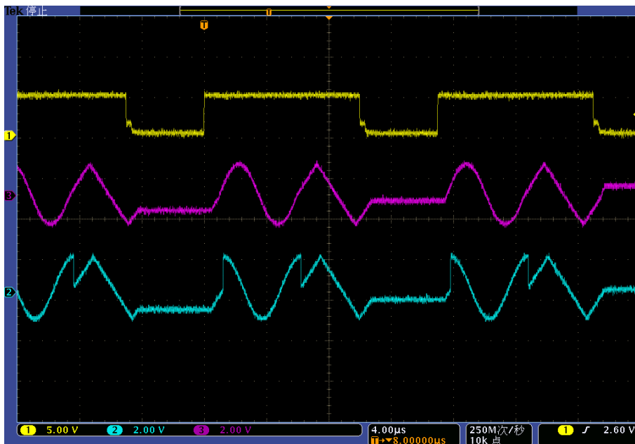
Fig. 4.29 Diagram of Arbitrary Trigger (Gate High)
