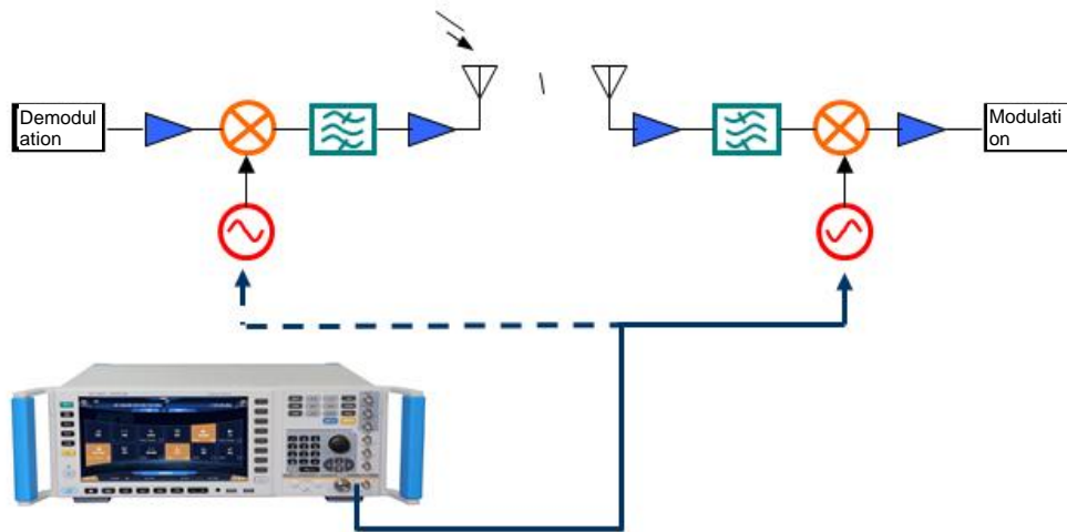
Fig. 2.15 Application of 1465 series signal generator in Local Oscillator Substitution
