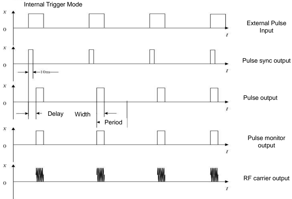
Fig. 4.17 Internal Trigger Mode
