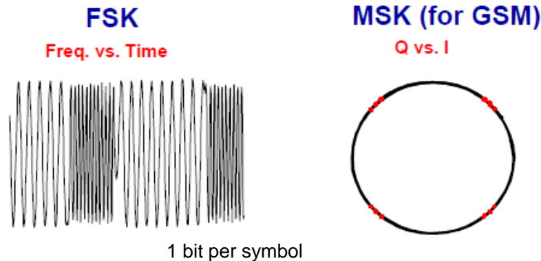
Attached Figure 9 MSK Modulation Method
