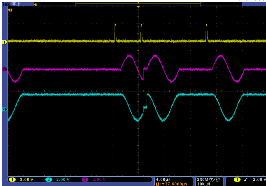
Fig. 4.27 Diagram of Arbitrary Trigger (Single/Real-time Repeated Trig)
