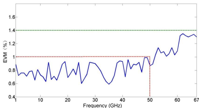
Fig. 2.8 Vector Modulation Accuracy
