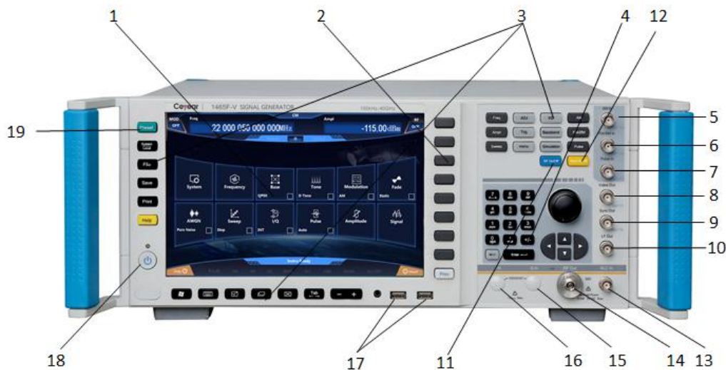
Fig. 3.11 Front Panel
