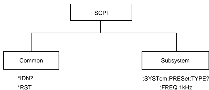
Figure 6.1 SCPI Types
