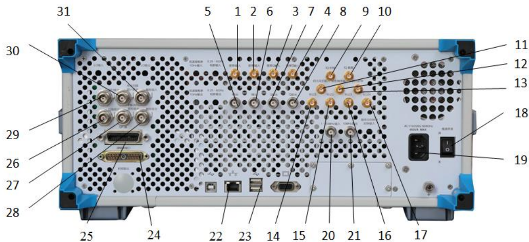
Fig. 3.12 Rear Panel
