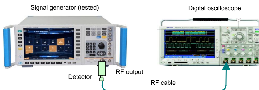
Figure 8.7 Pulse Modulation On-off Ratio Test
