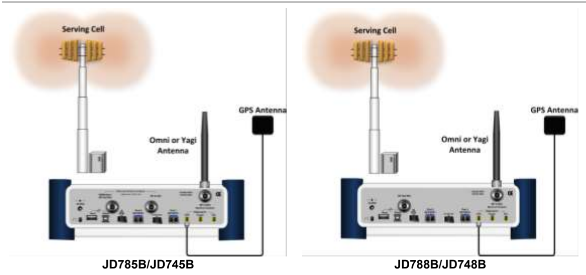
Figure 85 OTA connection
