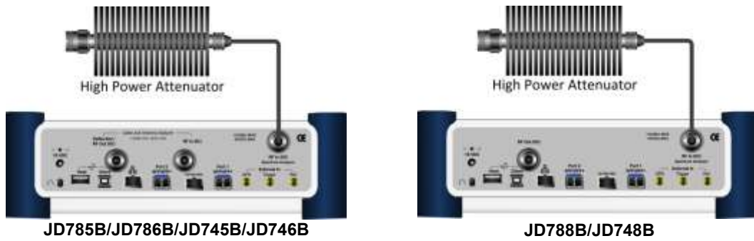
Figure 445 Direct connection
