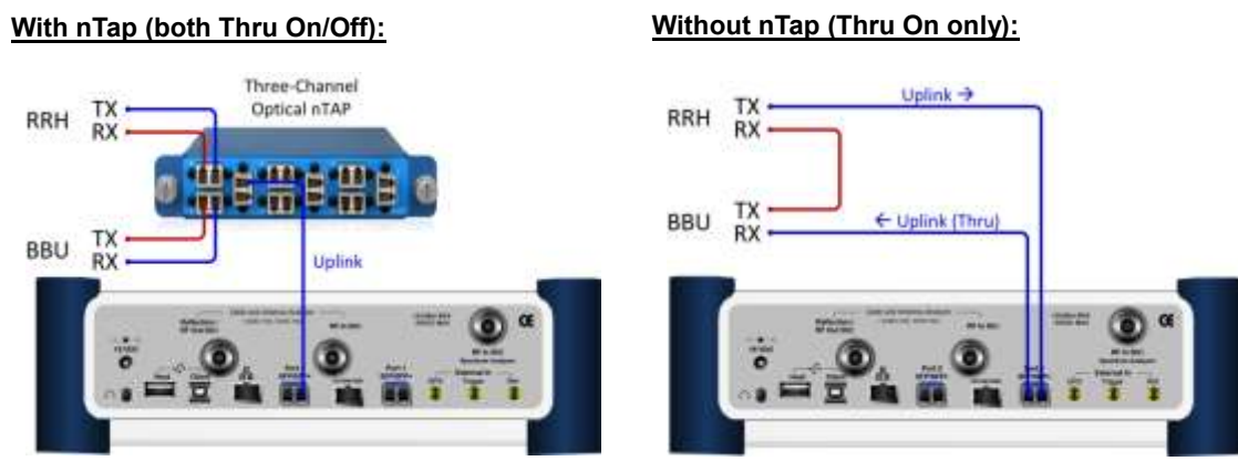
Figure 358 Connection diagram for PIM detection
