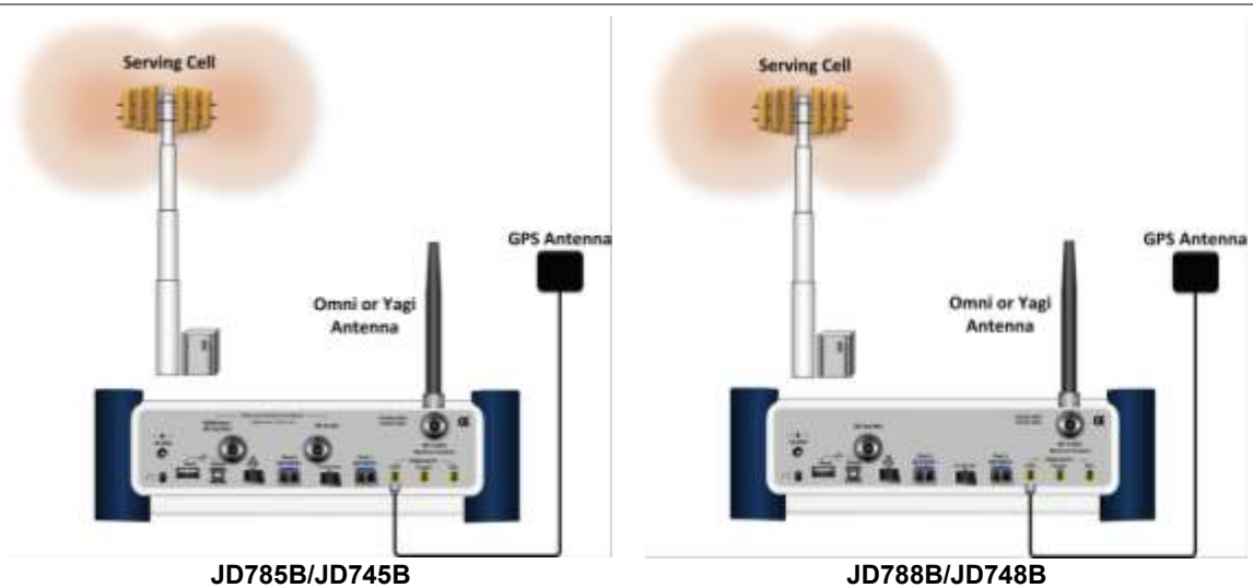
Figure 255 OTA connection
