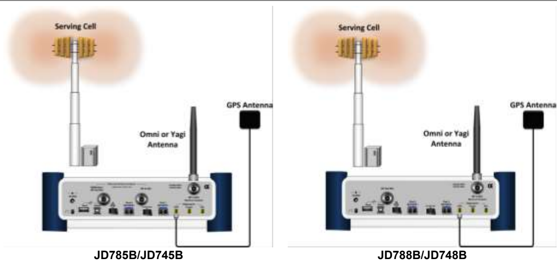
Figure 66 OTA connection
