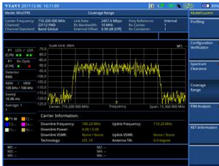
Figure 403 Example of coverage range in BBU emulation
