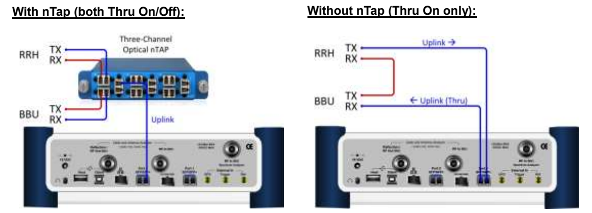
Figure 339 Connection diagram for interference analysis
