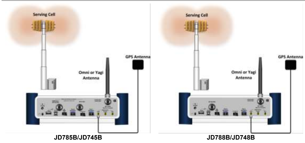
Figure 299 OTA connection
