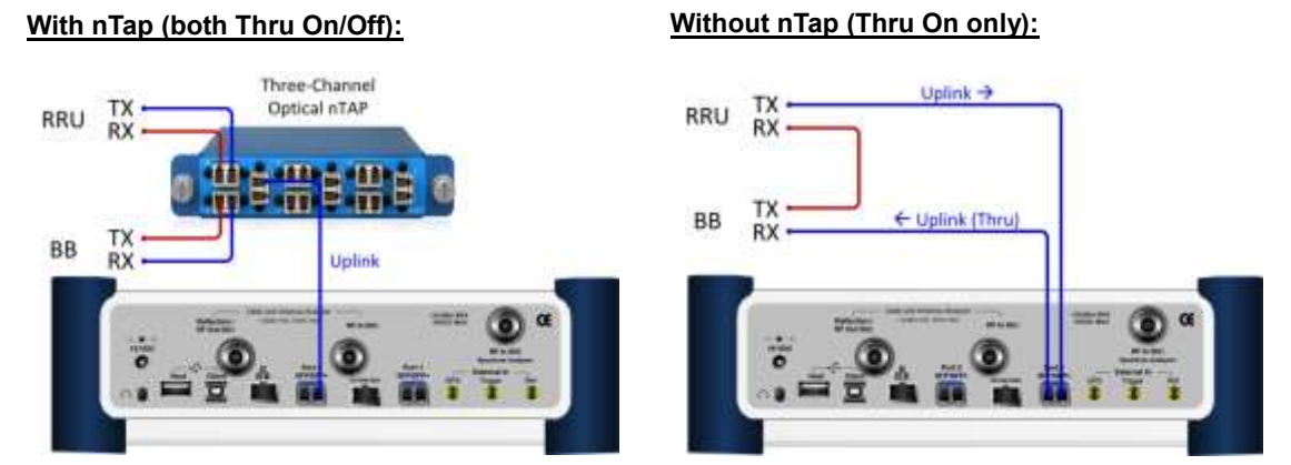
Figure 422 Connection diagram for PIM detection
