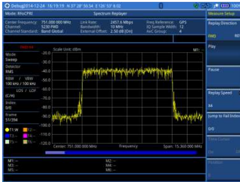
Figure 357 RFoCPRI spectrum replay
