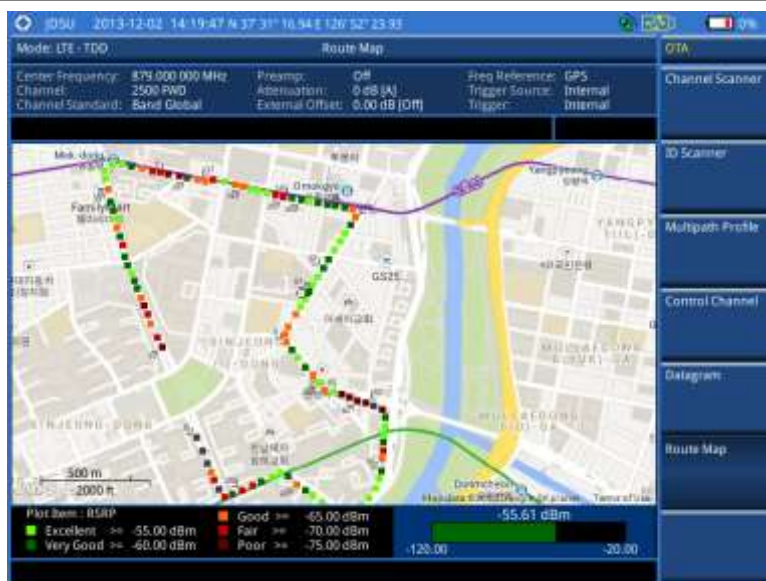
Figure 195 Route map measurement (RSRP) with LTE-TDD OTA signal analyzer
