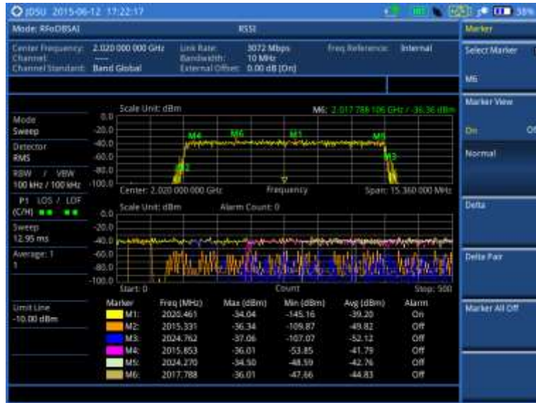
Figure 420 RFoBSAI interference measurement in RSSI
