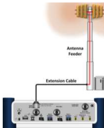
Figure 319 Connection for reflection measurement
