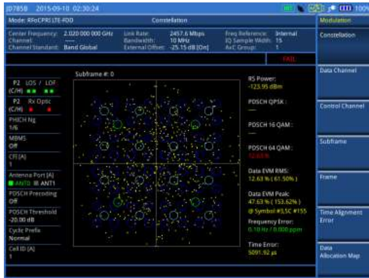
Figure 366 Constellation measurement with RFoCPRI LTE-FDD signal analyzer
