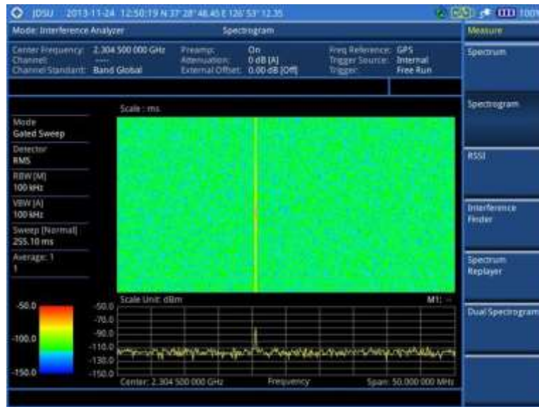
Figure 49 Interference measurement in spectrogram with gated sweep on
