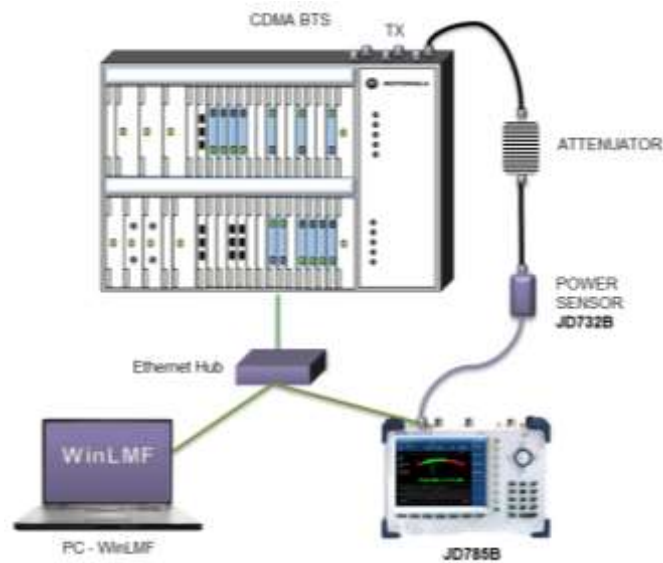
Figure 460 Using external power sensor
