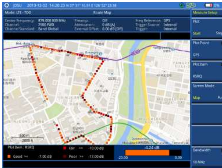
Figure 196 Route map measurement (RSRQ) with LTE-TDD OTA signal analyzer
