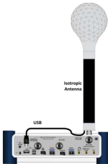
Figure 457 Connection using an isotropic antenna
