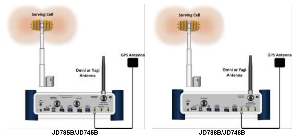
Figure 111 OTA connection
