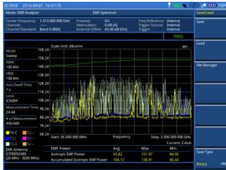
Figure 458 EMF spectrum measurement with EMF analyzer
