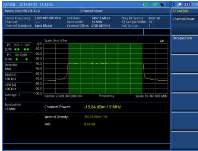
Figure 376 Channel power measurement with RFoCPRI LTE-TDD signal analyzer
