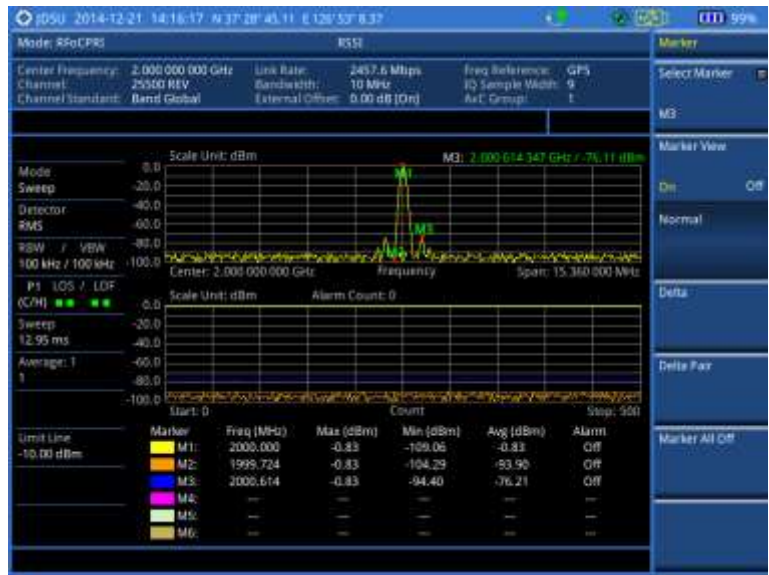
Figure 355 RFoCPRI interference measurement in RSSI
