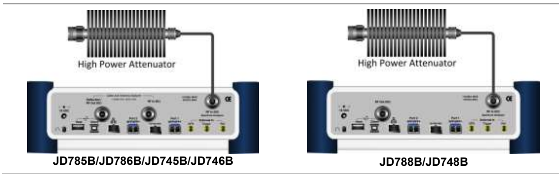
Figure 14 Direct connection
