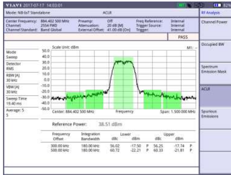
Figure 309 ACLR measurement with NB-IoT Standalone signal analyzer
