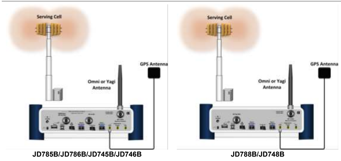
Figure 440 OTA connection
