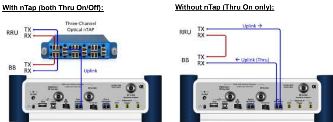
Figure 417 Connection diagram for interference analysis
