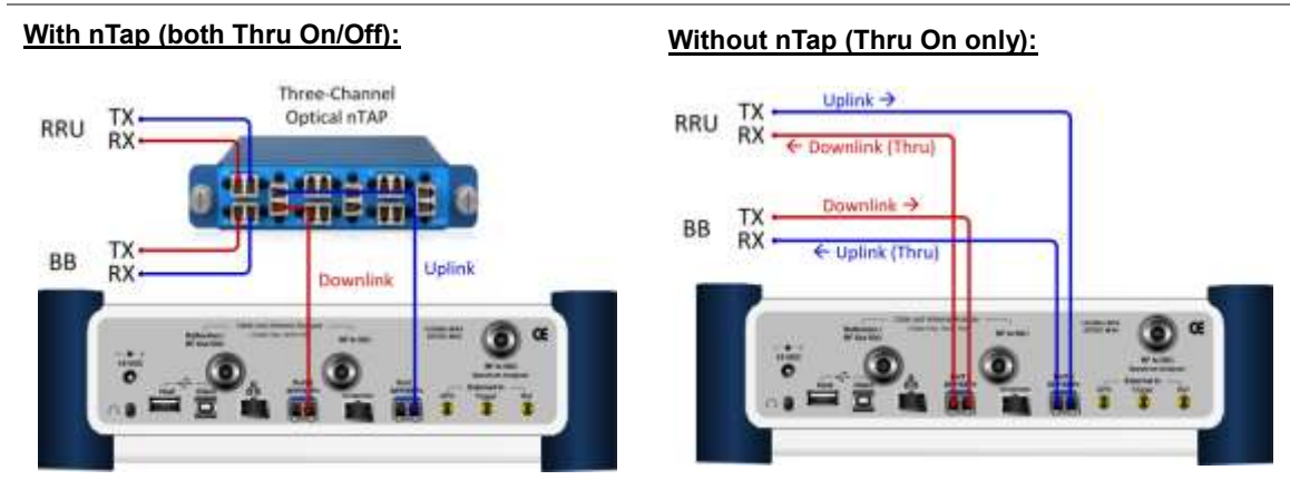
Figure 413 Connection diagram for Layer-2 monitoring mode
