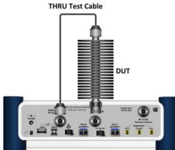
Figure 321 Connection for 2-port vector measurement
