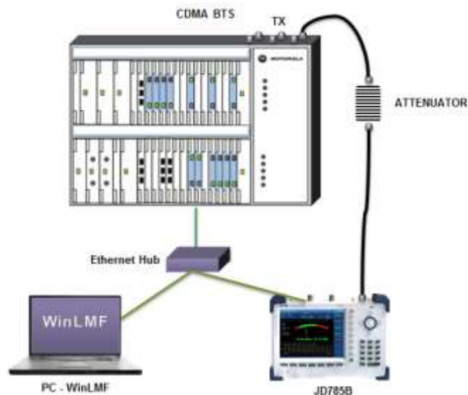
Figure 459 Using internal power sensor
