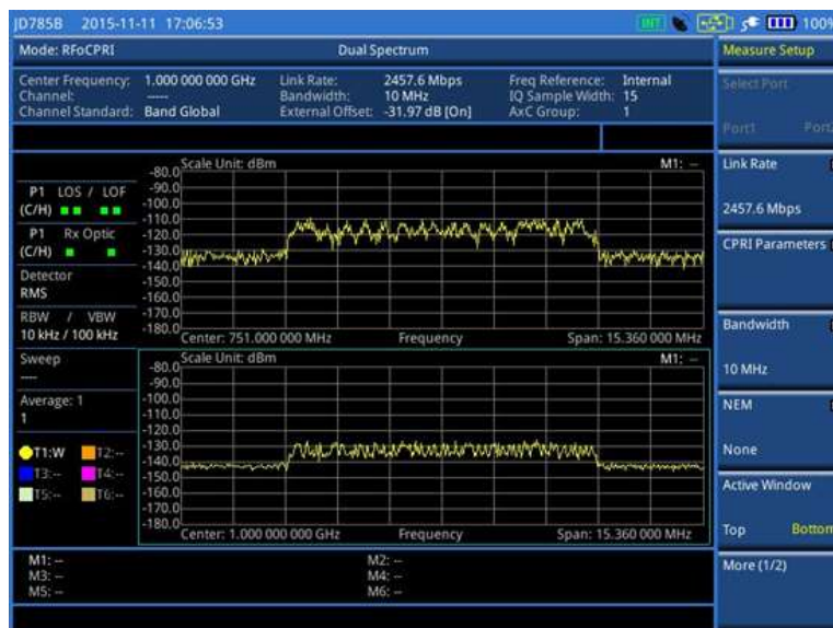
Figure 349 RfCPRI dual spectrum with dual active trace off
