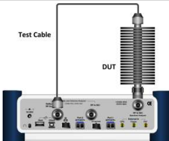
Figure 322 Connection for 2-port scalar measurement
