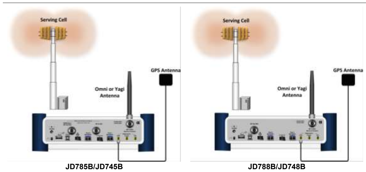
Figure 230 OTA connection
