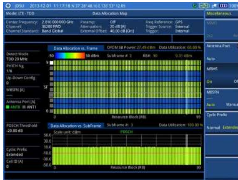
Figure 184 Data allocation map measurement with LTE-TDD signal analyzer (MBMS On)
