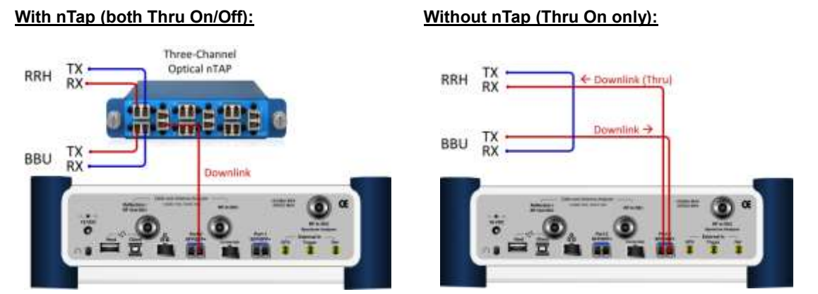
Figure 374 Connection diagram for downlink signal analysis
