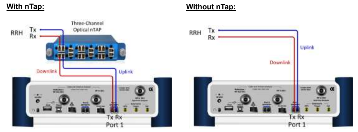
Figure 391 Term mode connection diagram
