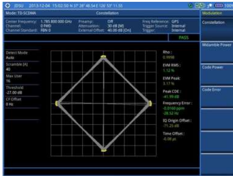
Figure 268 Constellation measurement with TD-SCDMA signal analyzer
