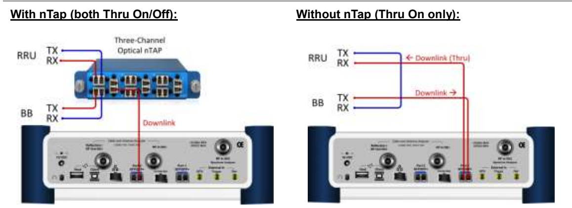
Figure 424 Connection diagram for downlink signal analysis
