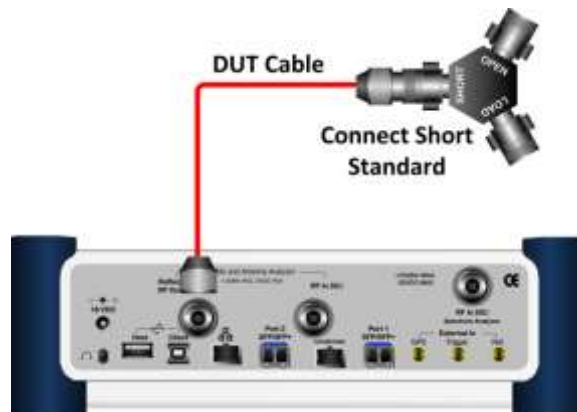
Figure 320 Connection for cable loss (1 port) measurement
