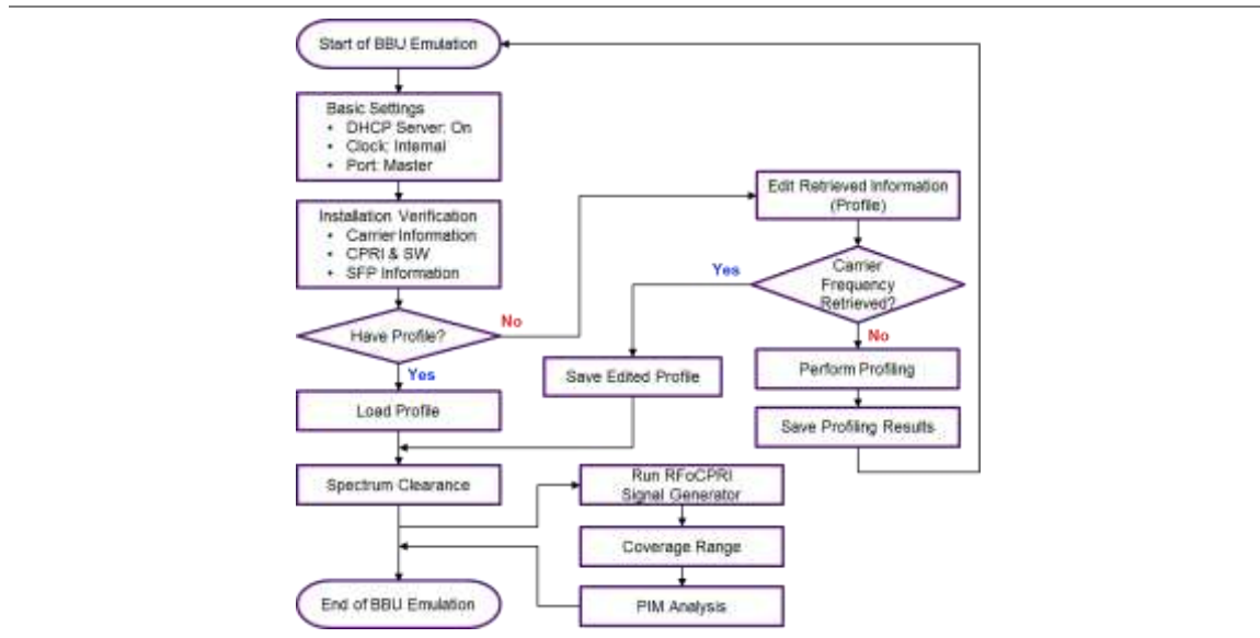
Figure 386 High-level workflow of BBU emulation
