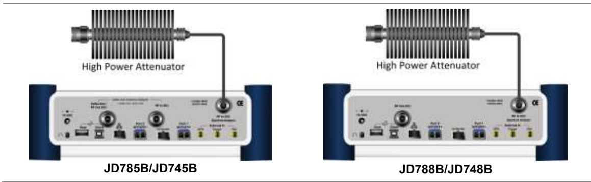
Figure 109 Direct connection
