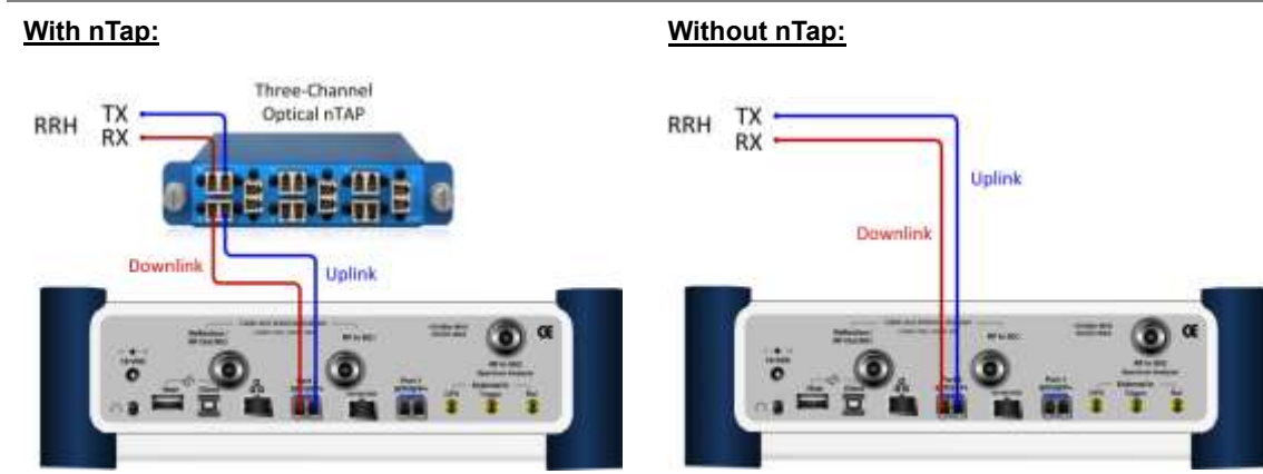
Figure 337 Connection diagram for Layer-2 term testing mode
