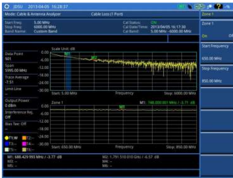
Figure 328 Cable loss (1 port) measurement with the zone enabled
