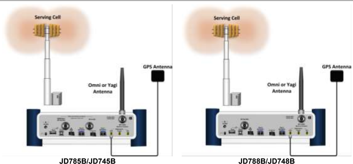
Figure 280 OTA connection
