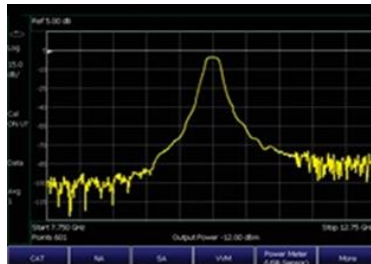
Characterize filter insertion loss
