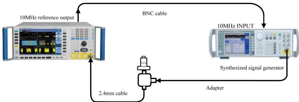
Fig. 8.10 Schematic diagram of frequency response test (3Hz ~ 50MHz)
