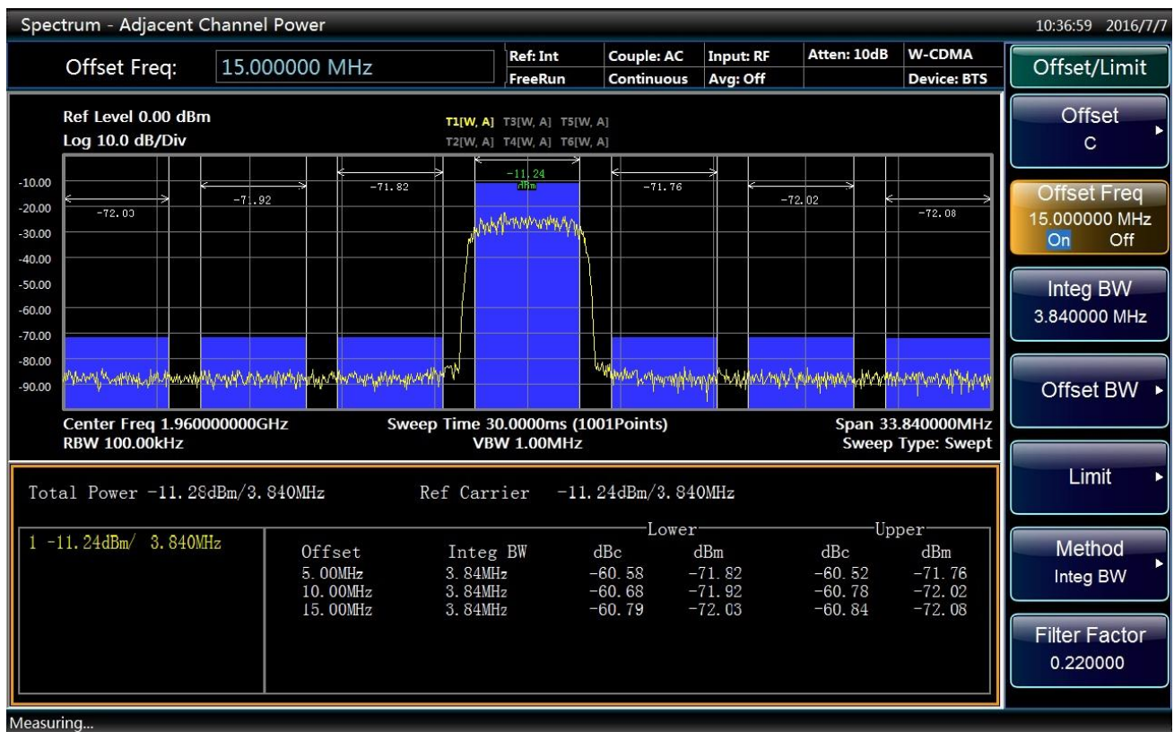
Fig.4.67 Measuring third adjacent channel
