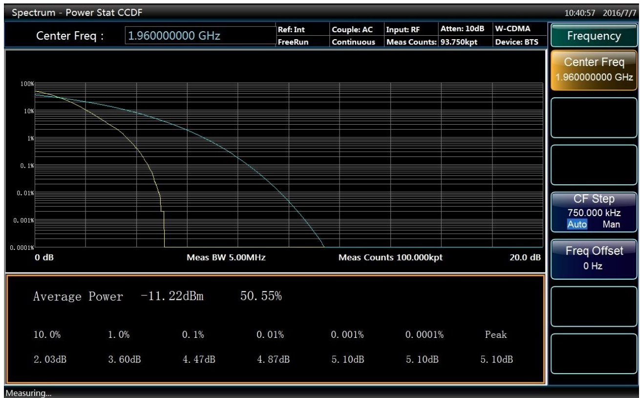
Fig. 4.70. Power Statistical Measurement
