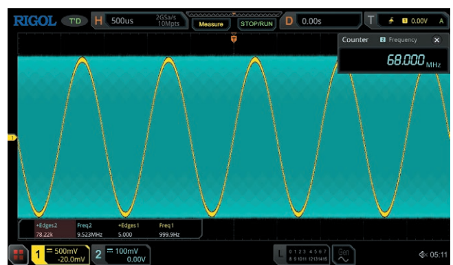
The ordinary 1 Mpts software measurement can no longer measure the accurate frequency of the high-frequency signal.
